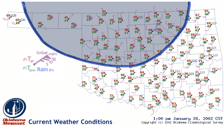
Figure 3. Weather conditions from the Oklahoma Mesonet at 1 p.m. on January 28 th . Air temperatures (degrees F) are in red to the upper left of each station model. Approximate southward progression of cold air is shown in the shaded region.
