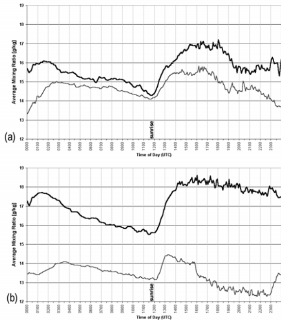
Figure 3. The diurnal cycle of the average mixing ratio (g/kg) at the Pawnee (thick trace) and Blackwell (thin trace) Mesonet stations during (a) 1-6 August 1994 and (b) 8-13 August 1994. The abscissa is time of day (0000-2355 UTC), and the ordinate is mixing ratio (12-19 g/kg).
