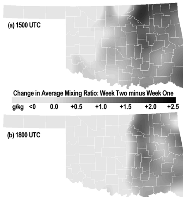
Figure 6. Using Mesonet data, change of the average mixing ratio at (a) 1500 UTC, and (b) 1800 UTC, between the week of 1-6 August 1994 and the week of 8-13 August 1994.
