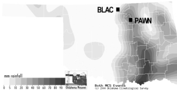
Figure 1. Combined rainfall from the MCS events of 5 August and 7 August 1994. The Blackwell (BLAC, 0 mm rainfall) and Pawnee (PAWN, 53 mm rainfall) Mesonet stations are noted.
