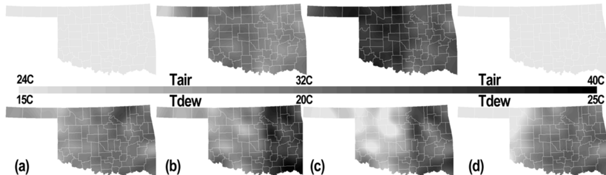
Figure 4. Mesonet air temperature (top) and dew point temperature (bottom) at (a) 1200 UTC on 11 August 1994; (b) 1600 UTC on 11 August 1994; (c) 2100 UTC on 11 August 1994; and (d) 1200 UTC on 12 August 1994.
