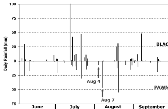
Figure 2. Daily Mesonet rainfall observations during June-September 1994. Each bar represents a 24-hour period ending at 0000 UTC. Values at BLAC appear above the zero line; those at PAWN appear below.
